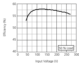
Efficiency by input voltage (@50 % load)
