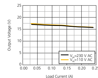
Load regulation
