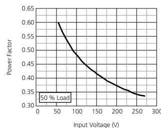
Power factor by input voltage (@50 % load)
